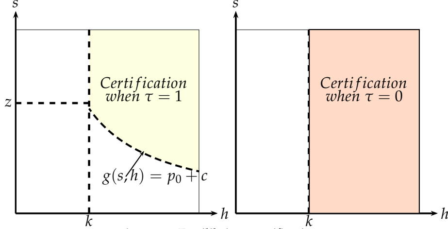
Figure 4: Equilibrium certification
